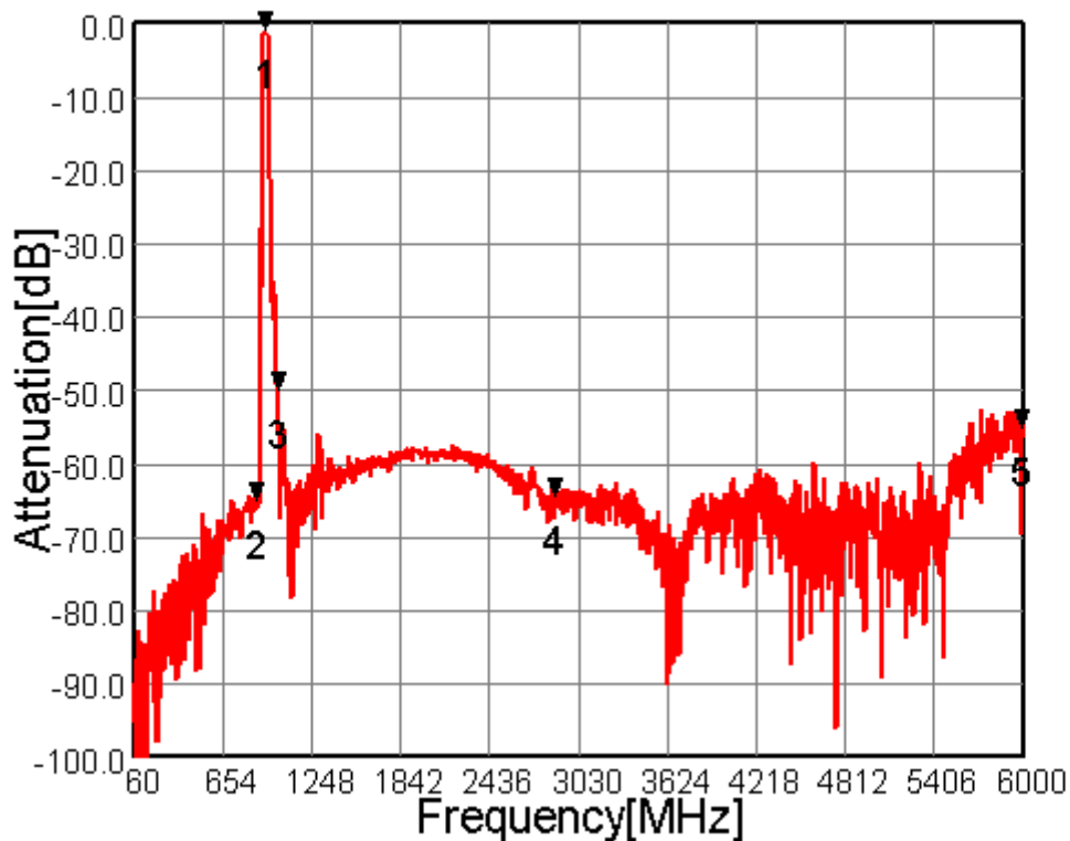
Fig.4 Wide-band Characteristics
