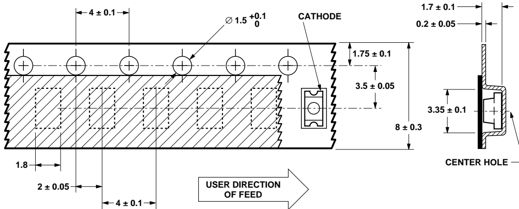
Figure 10. Tape Dimensions.
